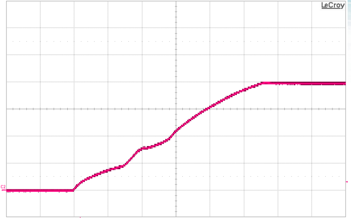
Figure 8: Output voltage startup waveform with 390µF hold-up capacitor, no load (115VAC, 60Hz) Vout (100V/div), Timebase: (500ms/div)
