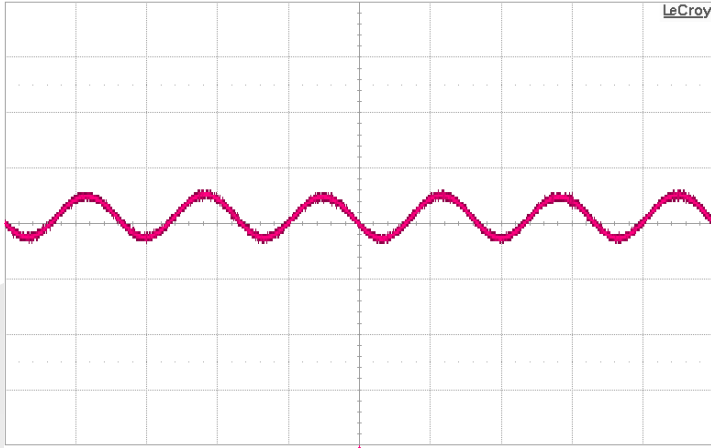
Figure 7: Output voltage ripple with 370µF Hold-up capacitor at full rated power (115VAC, 60Hz) Vout (10V/div), Timebase: (5ms/div)
