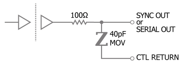
Figure 30: Internal circuitry for SYNC OUT and SERIAL OUT pins.
