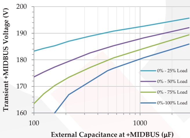
Figure 14: Instantaneous minimum value of +MIDBUS voltage during a (constant-current) load transient vs. external capacitance placed at +MIDBUS, shown at various load step amplitudes.
