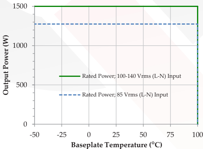
Figure 12: Rated steady state power vs. baseplate temperature. See Figure 11 for rated power vs. line voltage.
