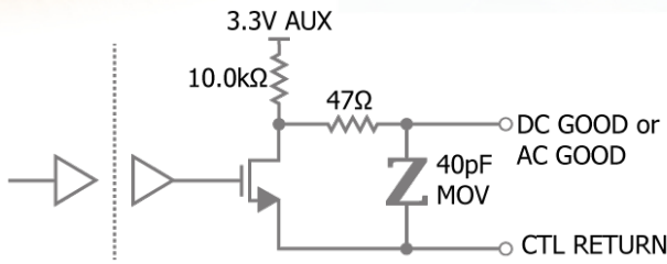
Figure 26: Internal circuitry for AC GOOD and DC GOOD pins.
