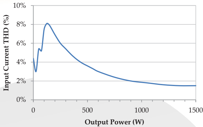
Figure 4: Input Current THD over full load range; input 3-phase 400 Hz 115 Vrms (L-N); includes external input filter module, part number MACF-115-3PH-UNV-HT.
