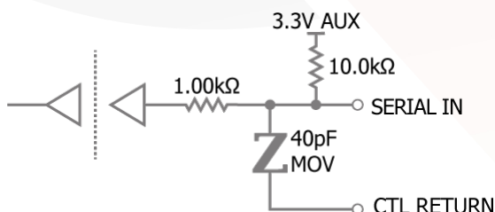
Figure 25: Internal circuitry for SERIAL IN pin.
