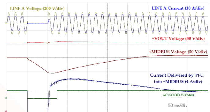
Figure 17: Response to 50 ms line interruption; 60 Hz; 1250 W power drawn from +VOUT pin; 7.5 mF total capacitance placed at +MIDBUS with series R || D network as shown in Figure 18.
